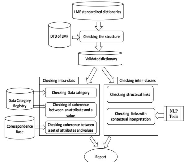
Figure 14: The approach overview for detecting anomalies in LMF-standardized dictionaries
