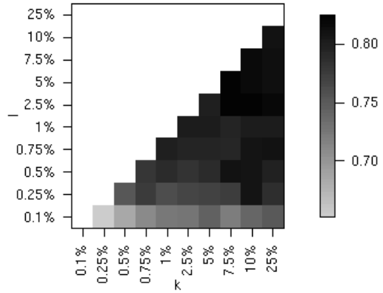
Figure 2: Parameter grid search by cross-validation.
