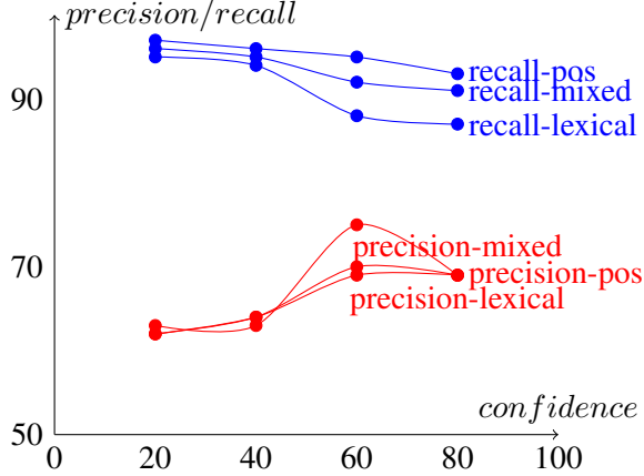
Figure 7: Precision/ Recall variance with Confidence
