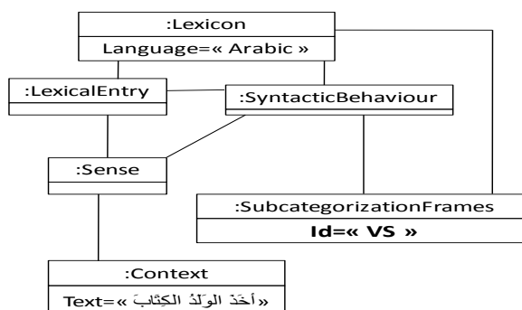
Figure 7: Illustration of the anomaly "incoherence between example and syntactic behavior"
