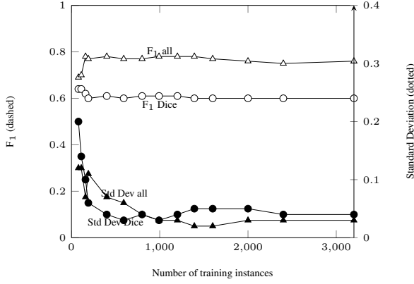
Figure 1: Training data sizes and corresponding F_1 and standard deviation.
