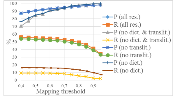
Figure 7: Latvian-English evaluation results using various resource configurations
