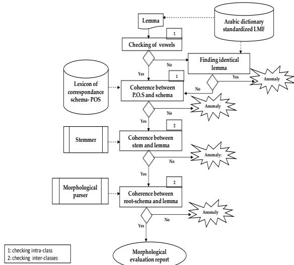
Figure 15: Morphological evaluation process
