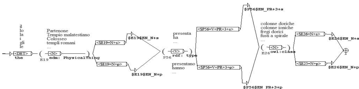
Figure 4: Translation FST with variables for identifying classes for subject, predicate and object
