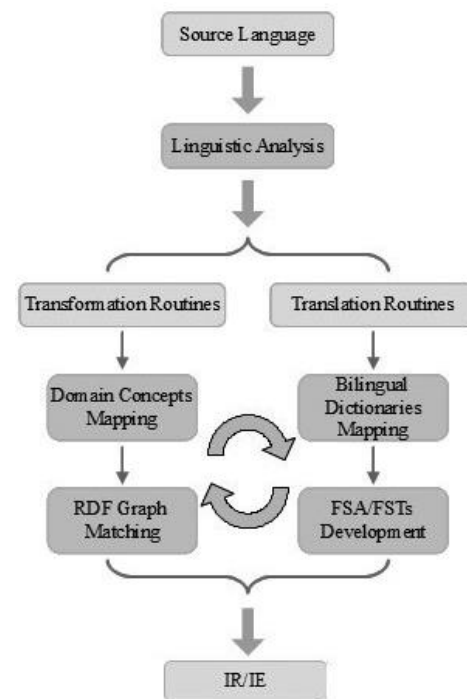
Figure 1: System Workflow
