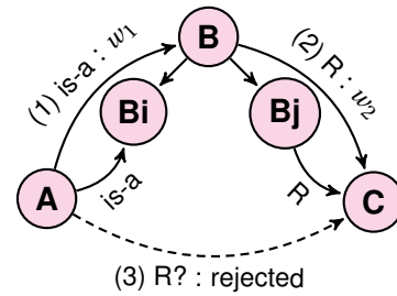
Figure 1: Triangular inference scheme with logical blocking based on the polysemy of B.
