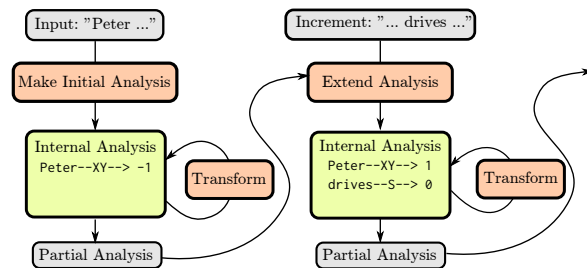
Figure 1: Incremental Parsing with jwcdg
