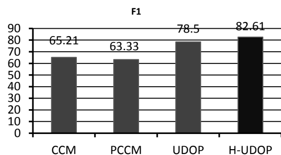
Figure 2. F1 scores for various models on WSJ-10.
