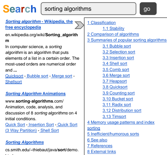
Figure 1: Search user interface showing a TOC along with the search results.
