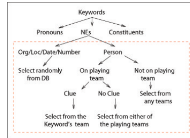
Figure 1: Distractor Selection Method
