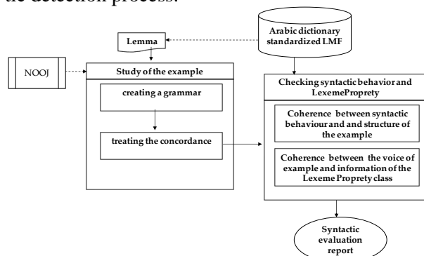
Figure 17: Syntactic evaluation process
