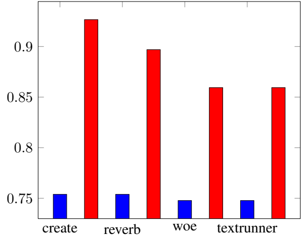
Figure 5: Comparison of CREATE performance with Reverb, WOE and TextRunner
